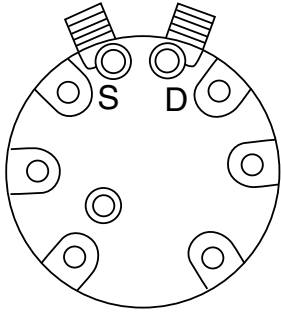
Sanden Cylinder Head FJ for all Types R12 & R134a
