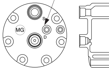
Sanden Cylinder Head MG w/o CP SD708, 709, 7H13 & 7H15 1" x 14 Tube O'Ring
