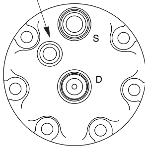
Sanden Cylinder Head KD SD708, 709, 7H13 & 7H15 Horizontal 3/4" x 7/8 O'Ring
