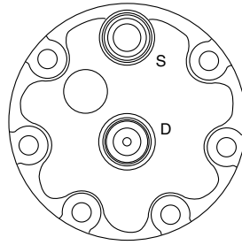
Sanden Cylinder Head KC SD7 3/4" x 7/8" Horizontal O'Ring
