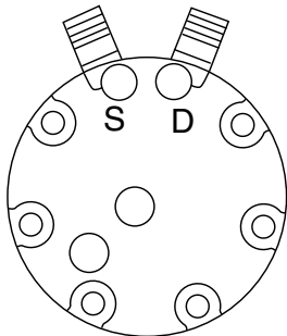
Sanden Cylinder Head JD SD 708-709, 7H15 Vertical O'Ring 3/4" x 7/8" w/o Charging Port
