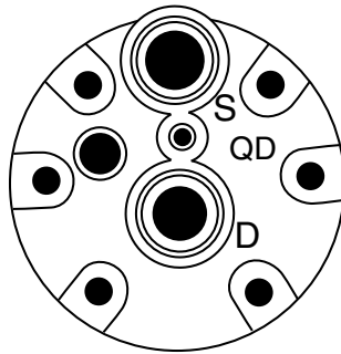
Sanden Cylinder Head QD SD709 Horizontal PAD
